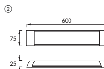
② FLATER LED 20W 4000K
