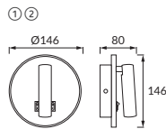
② OTELLO LED C 6W+3W BLACK
