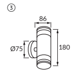
③ TARAS WLL 2xGU10 INOX
