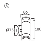
③ TARAS WLL 2xGU10 INOX
